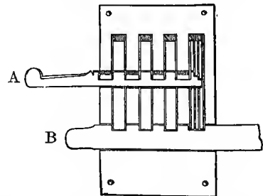
Larger Lock with Key. The key (A) lifts the wooden pegs which it touches, and thus allows the bar (B) below to be moved.
