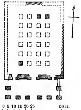
Synagogue at Kefr Bir'im in Galilee (Ground-Plan).
