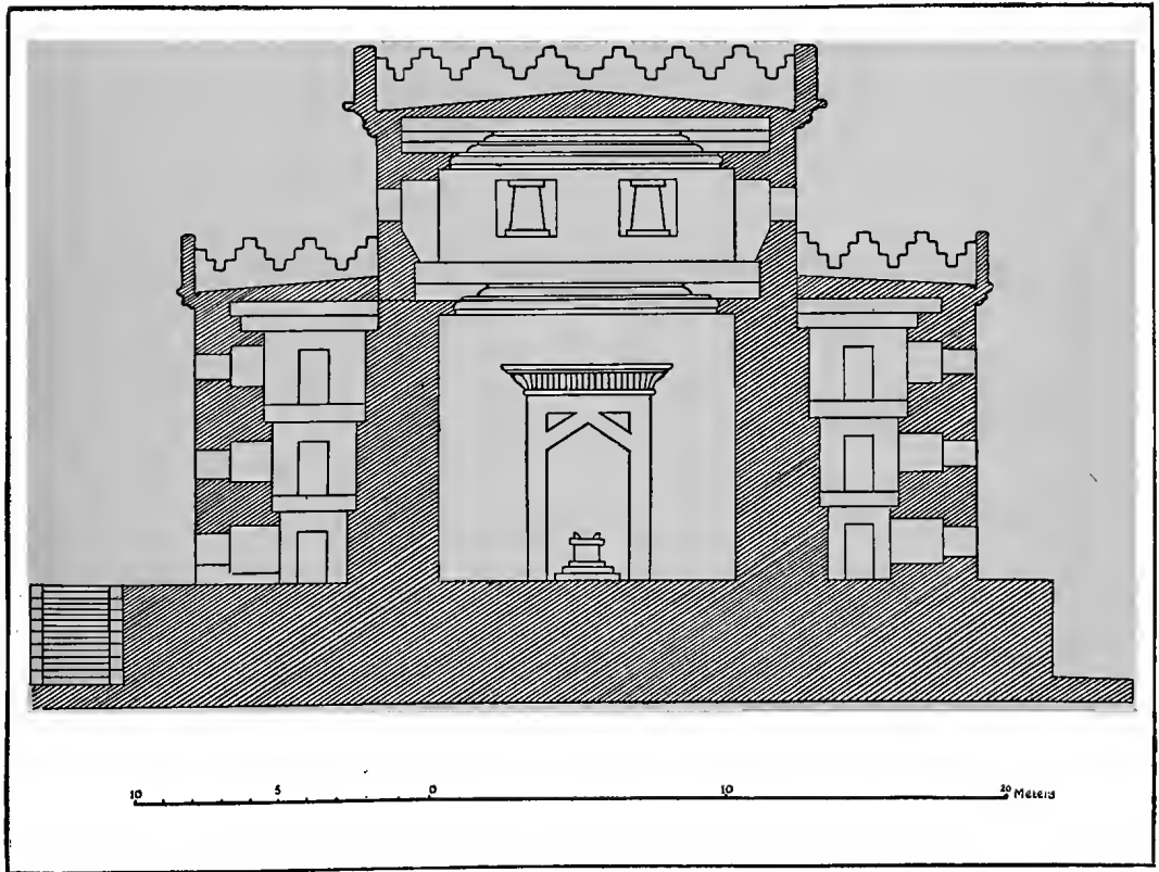
SOLOMON'S TEMPLE (AFTER STADE). FRONT ELEVATION SHOWING THE PROBABLE CONSTRUCTION OF THE SIDE CHAMBERS.
