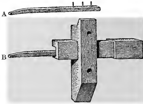
Lock and Key of a Palestinian Peasant's House. The key (A) lifts, by means of its pegs, three movable wedges in the lock (B), thus loosening the bolt.
